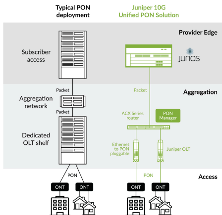
Figure 3: Legacy versus Juniper Unified PON solution
